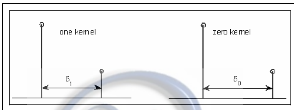
Gambar 2.3 Kernel. [8]
