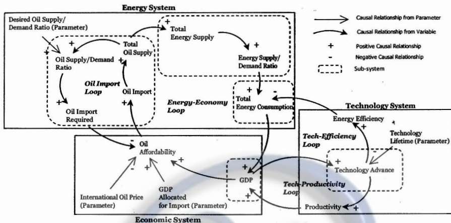
Fig 3. Key feedback loops of the model
