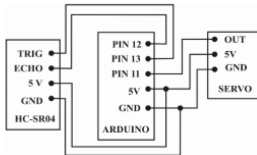
Image 6. Arduino Circuit
