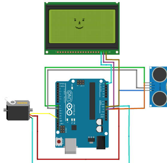
Image 7. Arduino IoT Schematic Circuit
