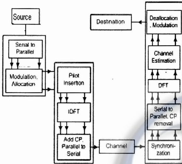
Fig. 1 Block Diagram of The Pilot Based OFDM System
