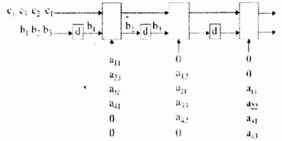
Fig. 4. Linear Systolic Architecture proposed by Mlovanovic
