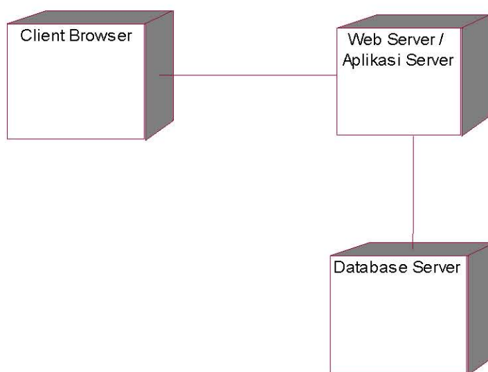
Gambar 5.3 Deployment diagram
