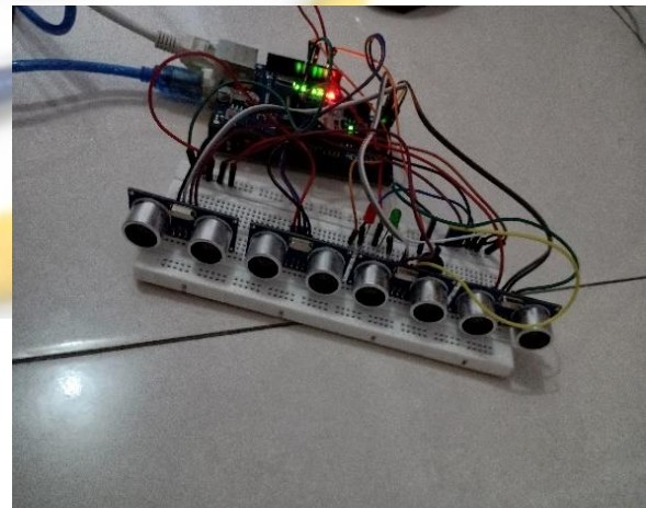
Fig.5 Ultrasonic Implementation
