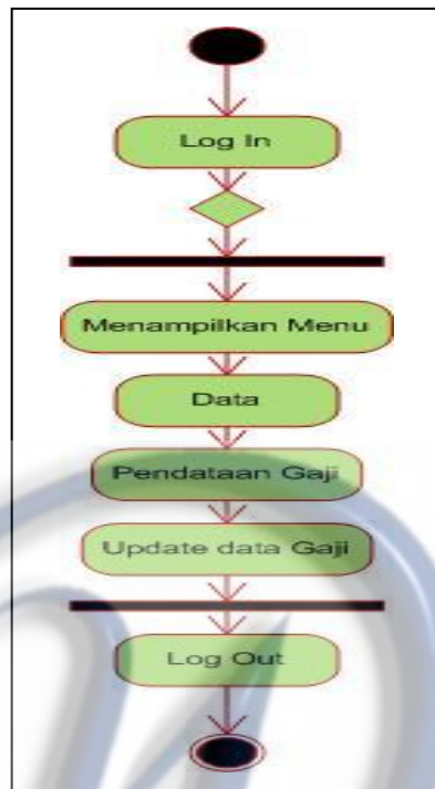
Gambar 4.9 Activity Diagram Edit data Gaji Karyawan
